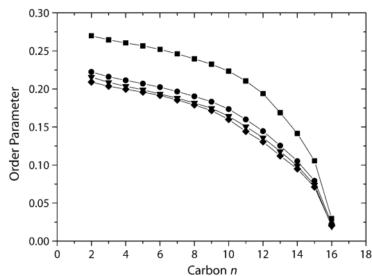
Figure 2. Smoothed order parameter profiles determined from solid-state 2 H NMR experiments of sn -1 chain perdeuterated [D 31 ]POPC (◆) and 1:4 (mol/mol) mixtures of 10b /[D 31 ]POPC (●), 11 /[D 31 ]POPC (■) and 17 /[D 31 ]POPC membranes (▼) at a temperature of 303 K and a water content of 40 wt.-%.
