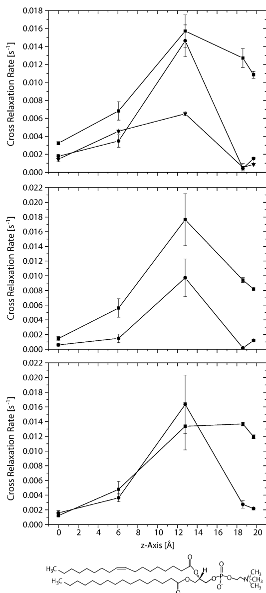
Figure 3. ^1\text{H} NOESY NMR cross-relaxation rates ( \text{s}^{-1} ) between molecular segments of the lipophilic nucleosides and segments of POPC molecules in the membrane as a function of the coordinates obtained from a molecular dynamics simulation of pure POPC membranes. [68] Top: Distribution of the 6-H proton of the uracil moiety of 10b (●) and 11 (■) and the 8-H proton of the adenine nucleobase of 17 (▼) with respect to the membrane normal; middle: localization of the 5-H proton of the uracil nucleobase of 10b (●) and 11 (■) and bottom: distribution of the 1'-H proton of the ribose moiety of 10b (●) and 11 (■) within the POPC matrix.
