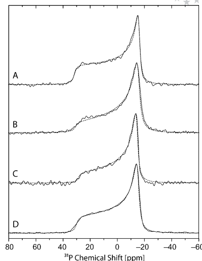
Figure 1. 31 P NMR spectra of pure POPC membranes (D) and of POPC in the presence of 11 (20 mol-%) (A), 10b (B) and 17 (C). All measurements were carried out at a water content of 40 wt.-% and a temperature of 30 °C. The dotted lines represent the best-fit simulations of the spectra.
